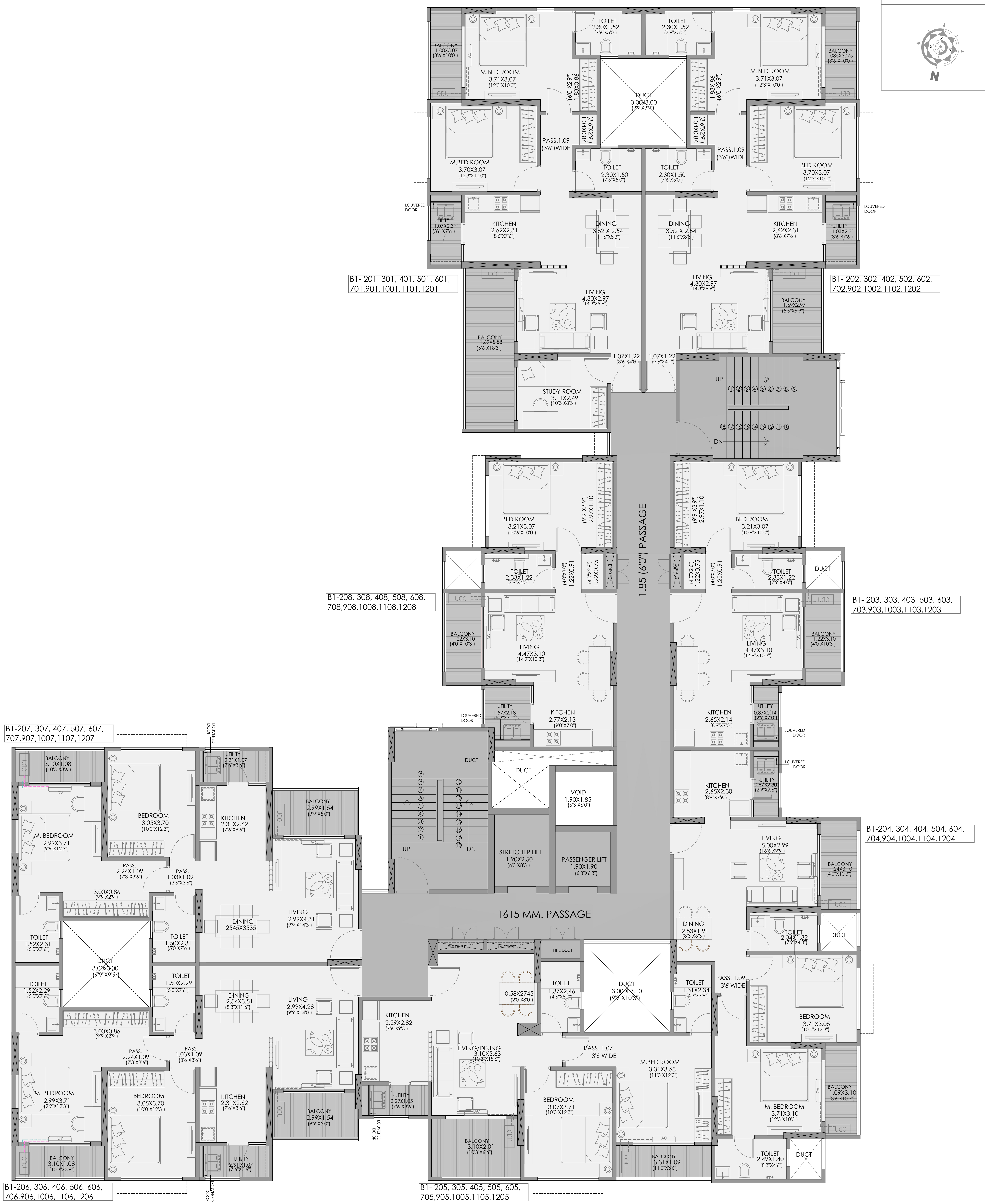
TYPICAL FLOOR PLAN FOR TOWER 'B1'
